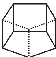
Prisma Pentagon
