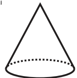
Kon
