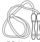
Tali skipping
